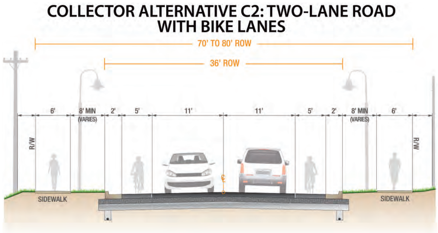
Figure 1.03-5 Collector Alternative C2
