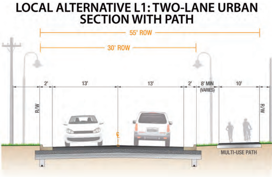
Figure 1.03-6 Local Alternative L1
