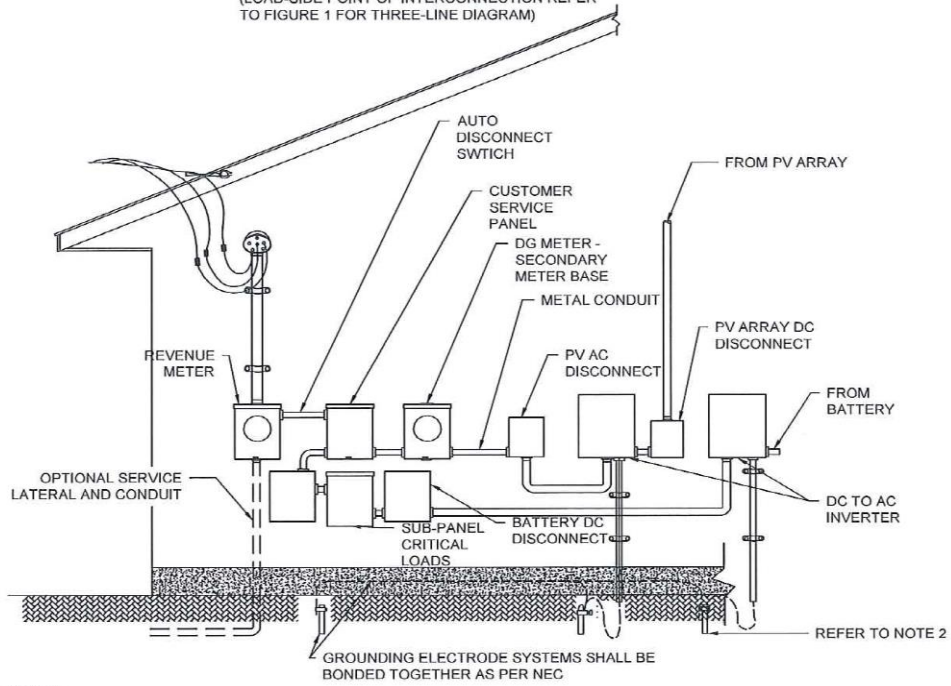
FIGURE 4 TYPICAL 120/240-VOLT, SINGLE-PHASE PHOTOVOLTAIC (PV) SYSTEM (LOAD-SIDE POINT OF INTERCONNECTION REFER TO FIGURE 1 FOR THREE-LINE DIAGRAM)
